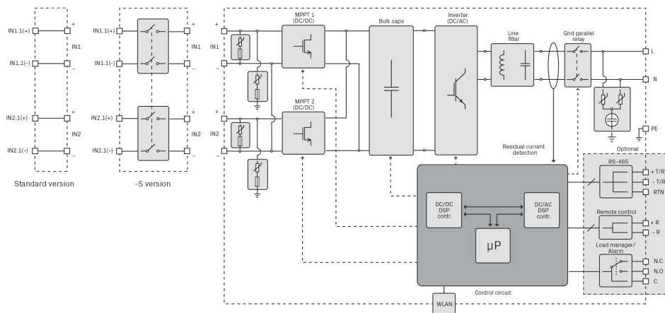
UNO-DM-6.0-TL-PLUS-Q string inverter block diagram
